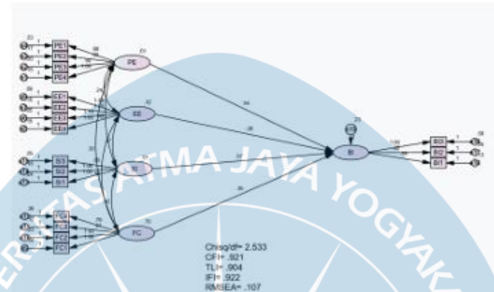
Figure 4. Unstandardised Estimate
