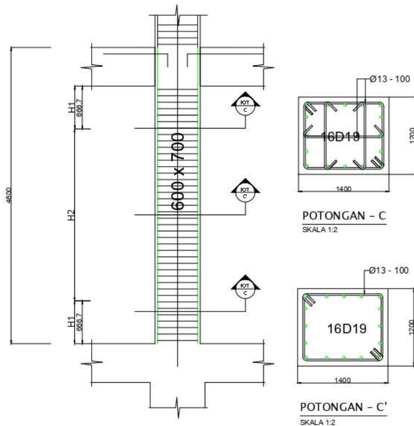
DETAIL KOLOM K2C SKALA 1: 7
