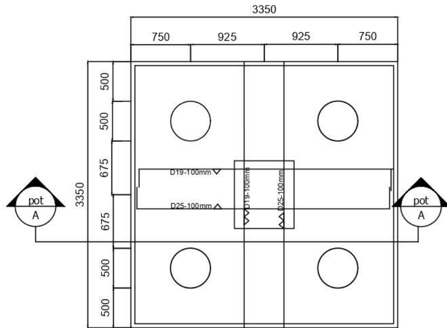
DETAIL PC 1 SKALA 1: 6
