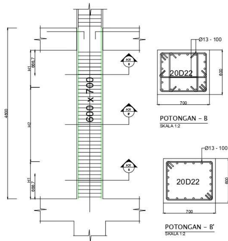
DETAIL KOLOM K2B
