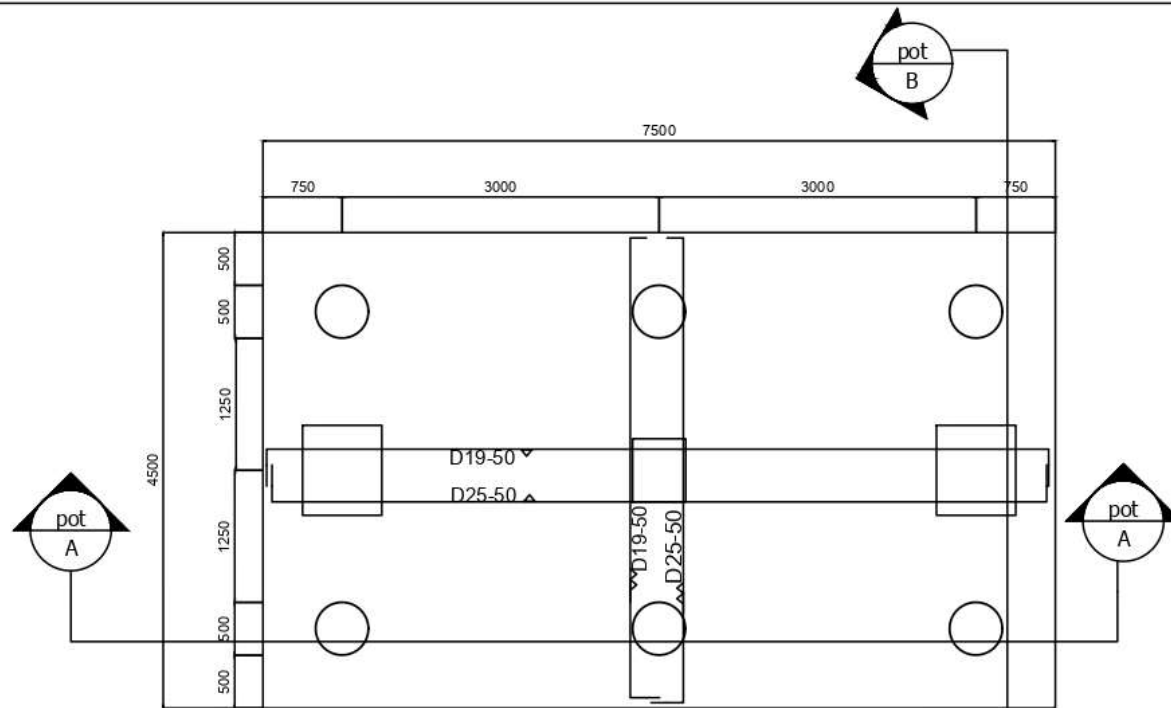
DETAIL PC 4 SKALA 1: 4
