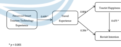
Figure 3. Hypothesis path analysis.
