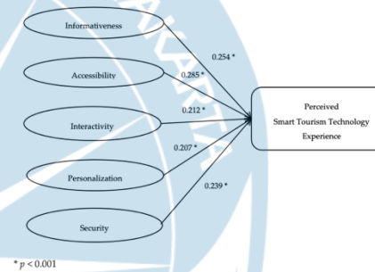
Figure 2. Structure model analysis of first-order variables.
