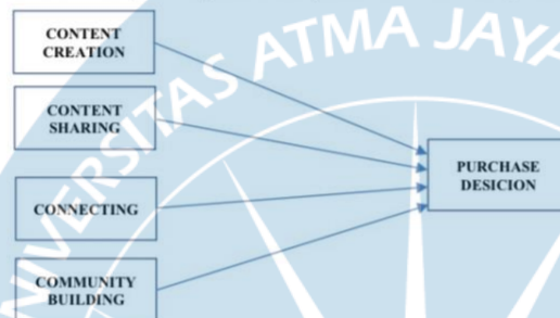
Figure 1. Conceptual Framework
