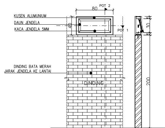
DETAIL BOUVEN KM
