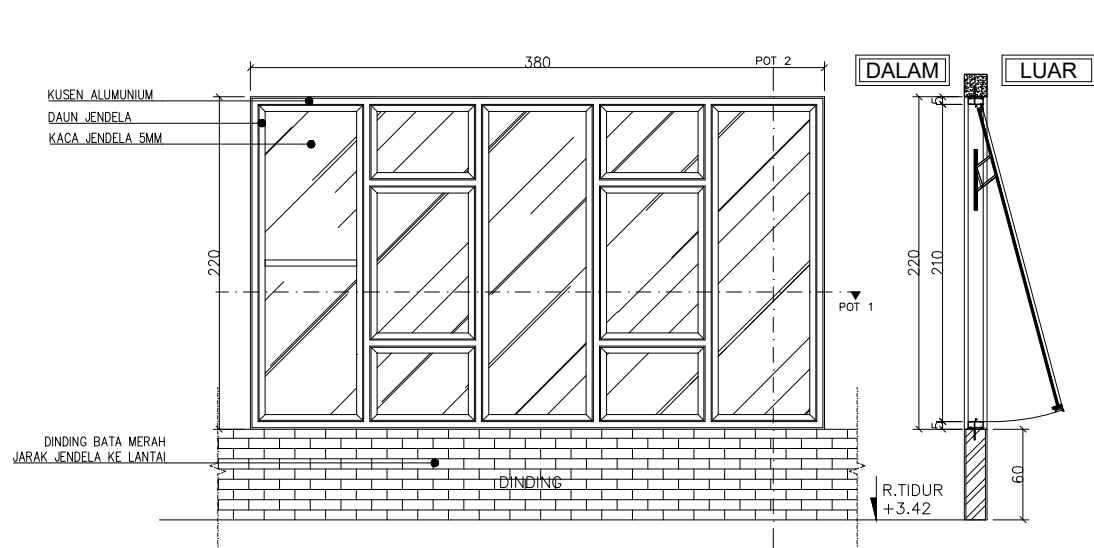
DETAIL JENDELA Skala 1: 50
