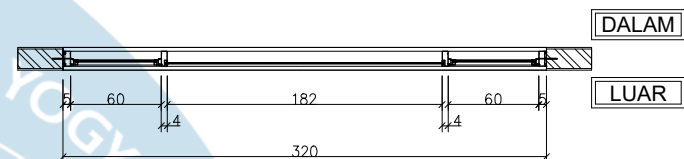
DETAIL JENDELA Skala 1: 50
