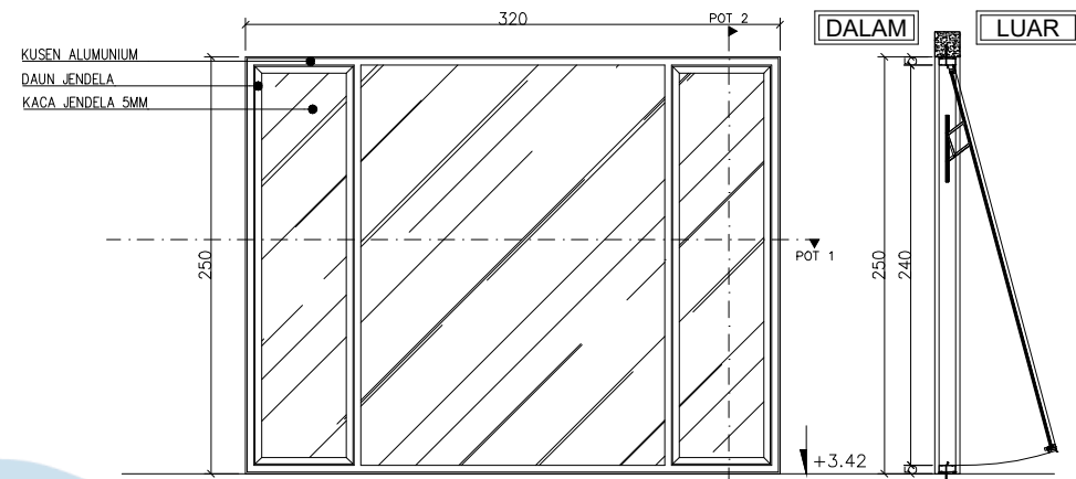
DETAIL JENDELA Skala 1: 50
