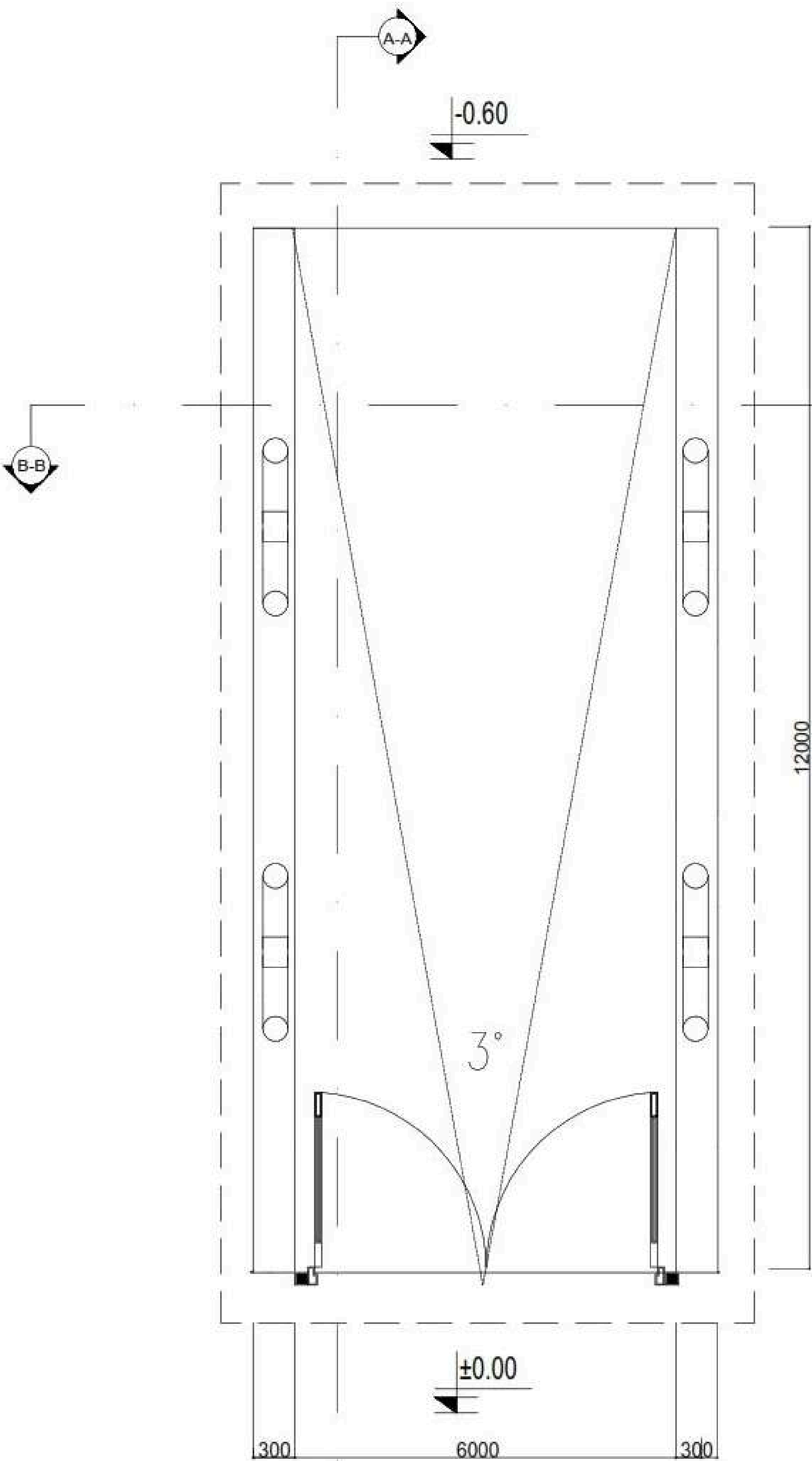
DENAH ENTRANCE SCALE 1:20
