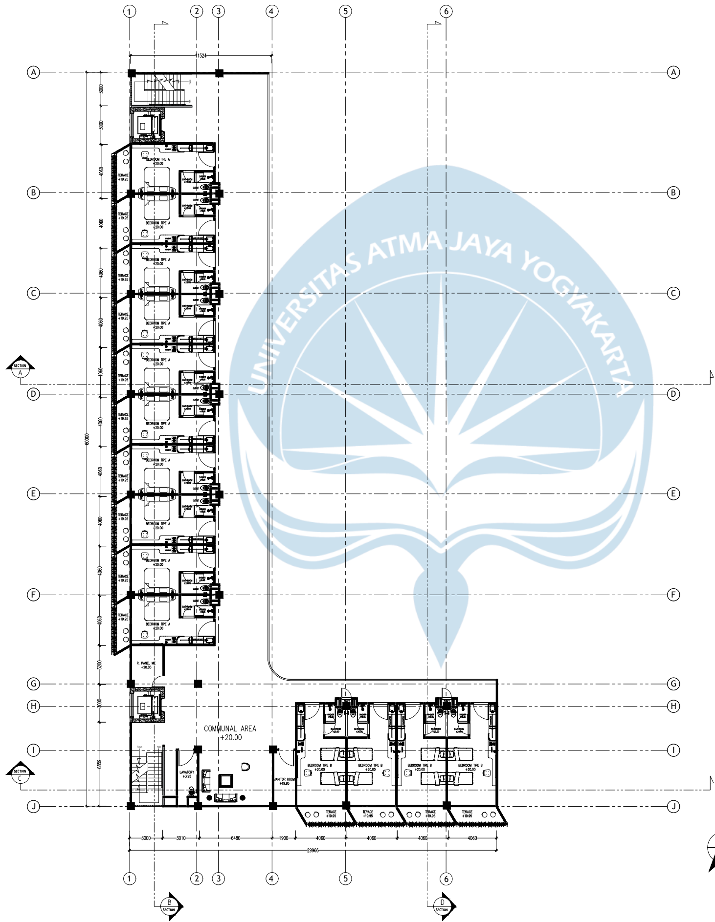
DENAH LANTAI 6 SCALE 1 : 100
