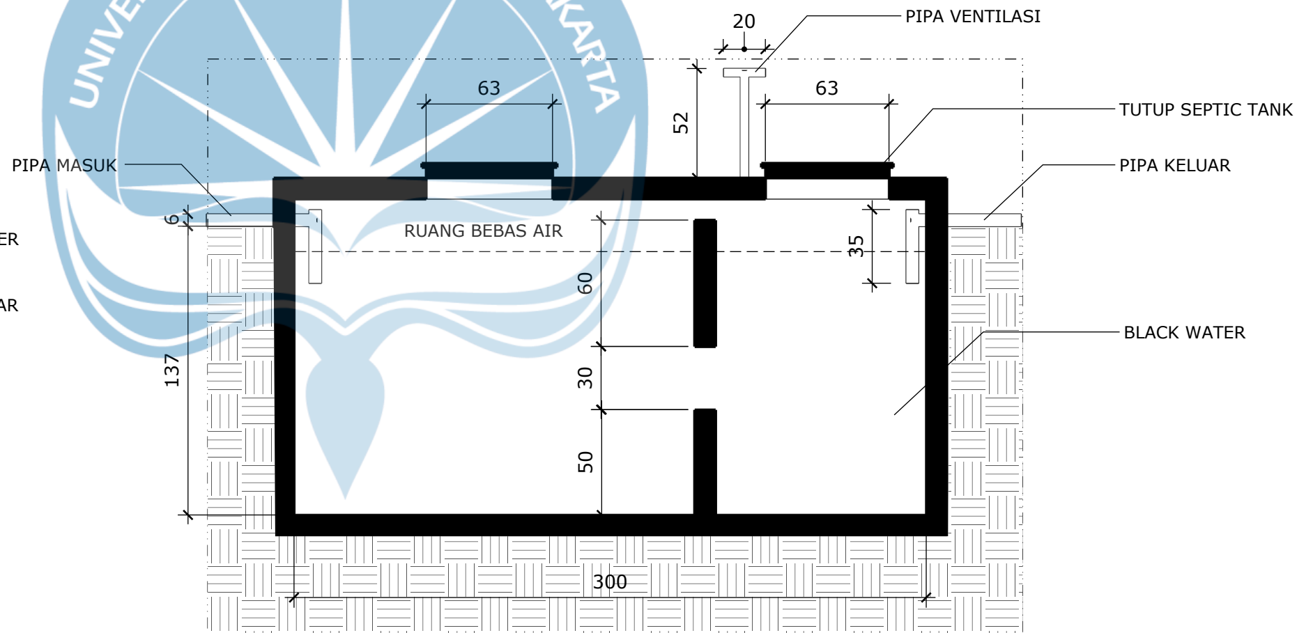
POTONGAN SEPTIC TANK 1:25
