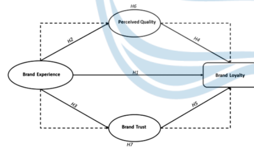
Figure 1. Proposed theoretical model
