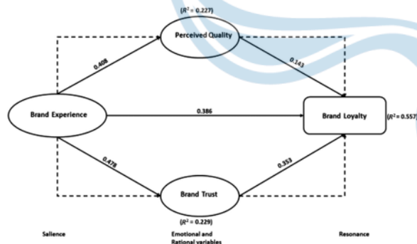
Figure 2. General model resolution by smart- PLS algorithm
