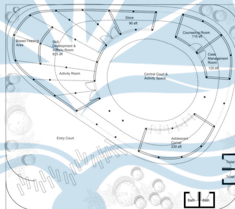
Gambar 2. 8 Beyond Survival Floor Plan
