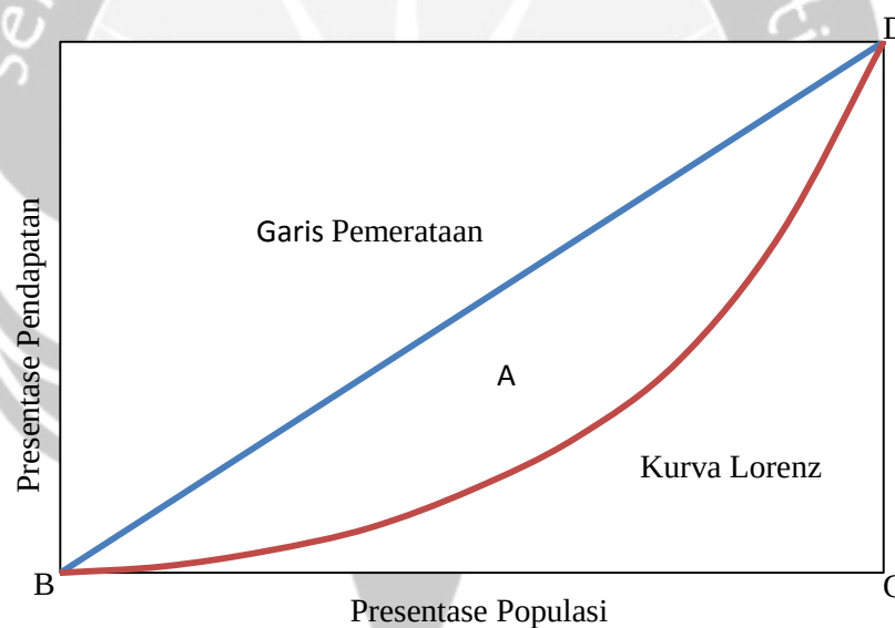
Gambar 2.2 Kurva Lorenz
