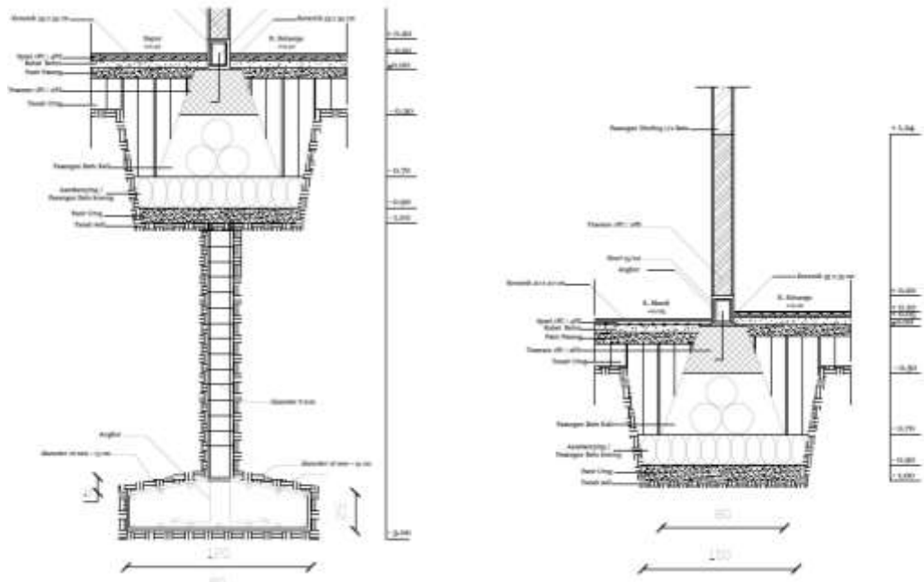
Gambar 7.5.1 Detail Pondasi
